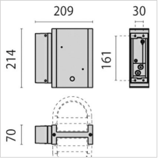
000400 Wall bracket 21
